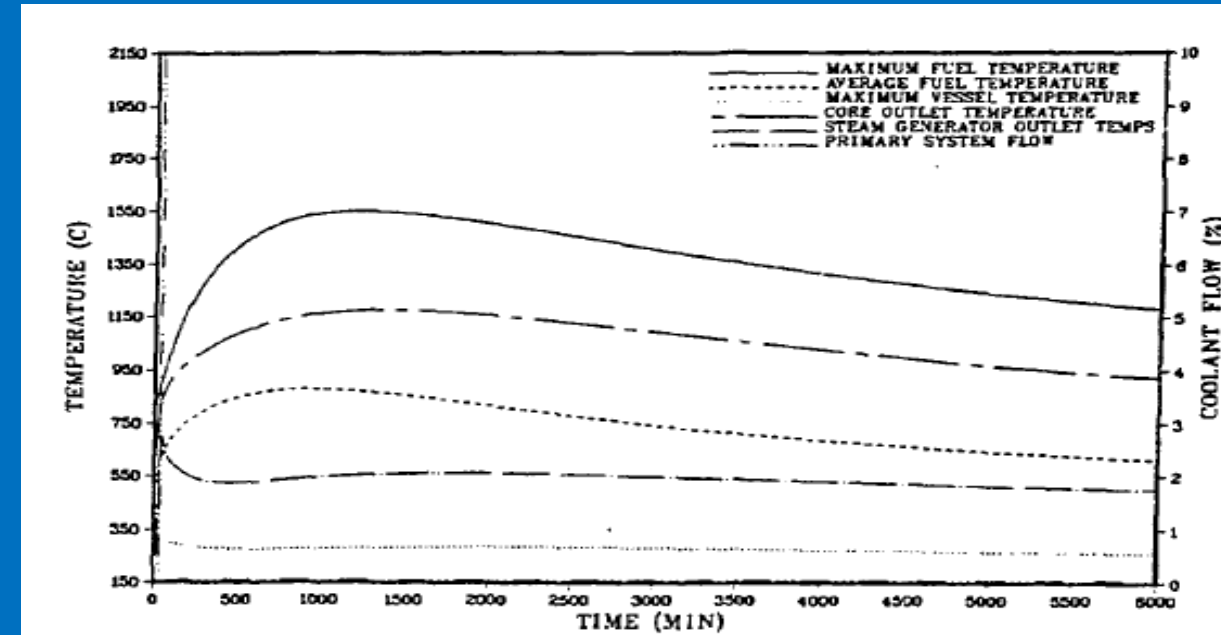
LOFC with depressurization and loss of feedwater
