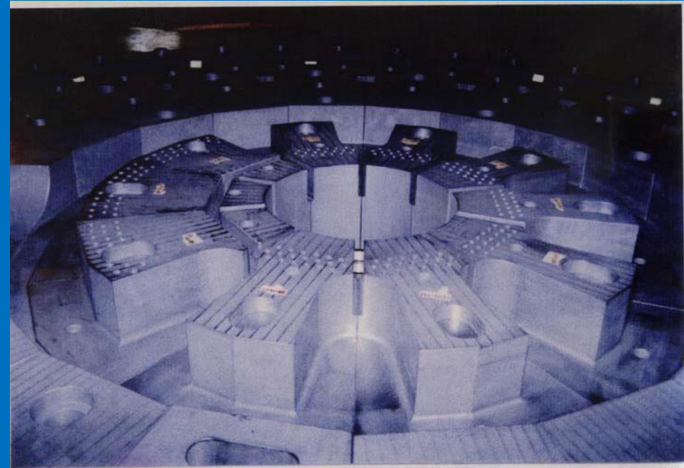
Top of the graphite core of HTR-10
